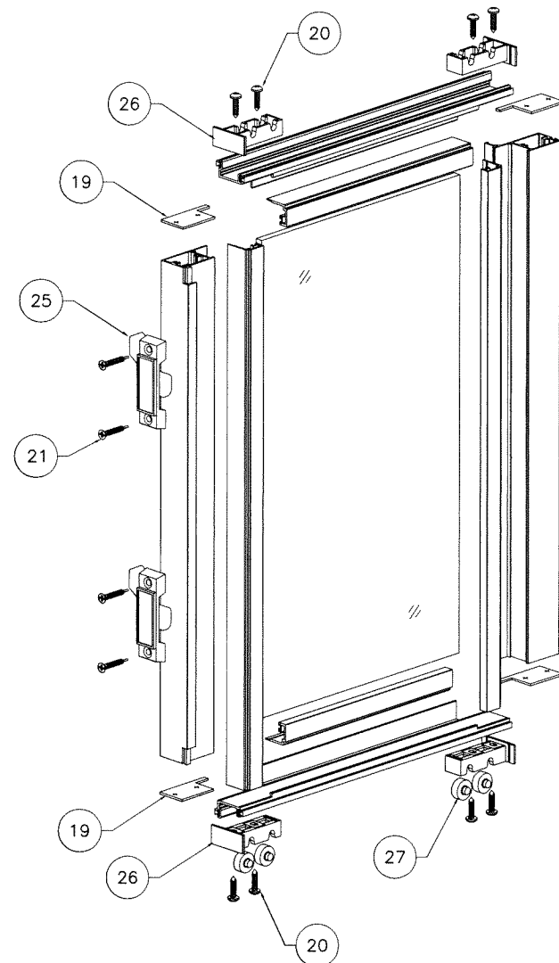
VENT ASSEMBLY DETAIL
