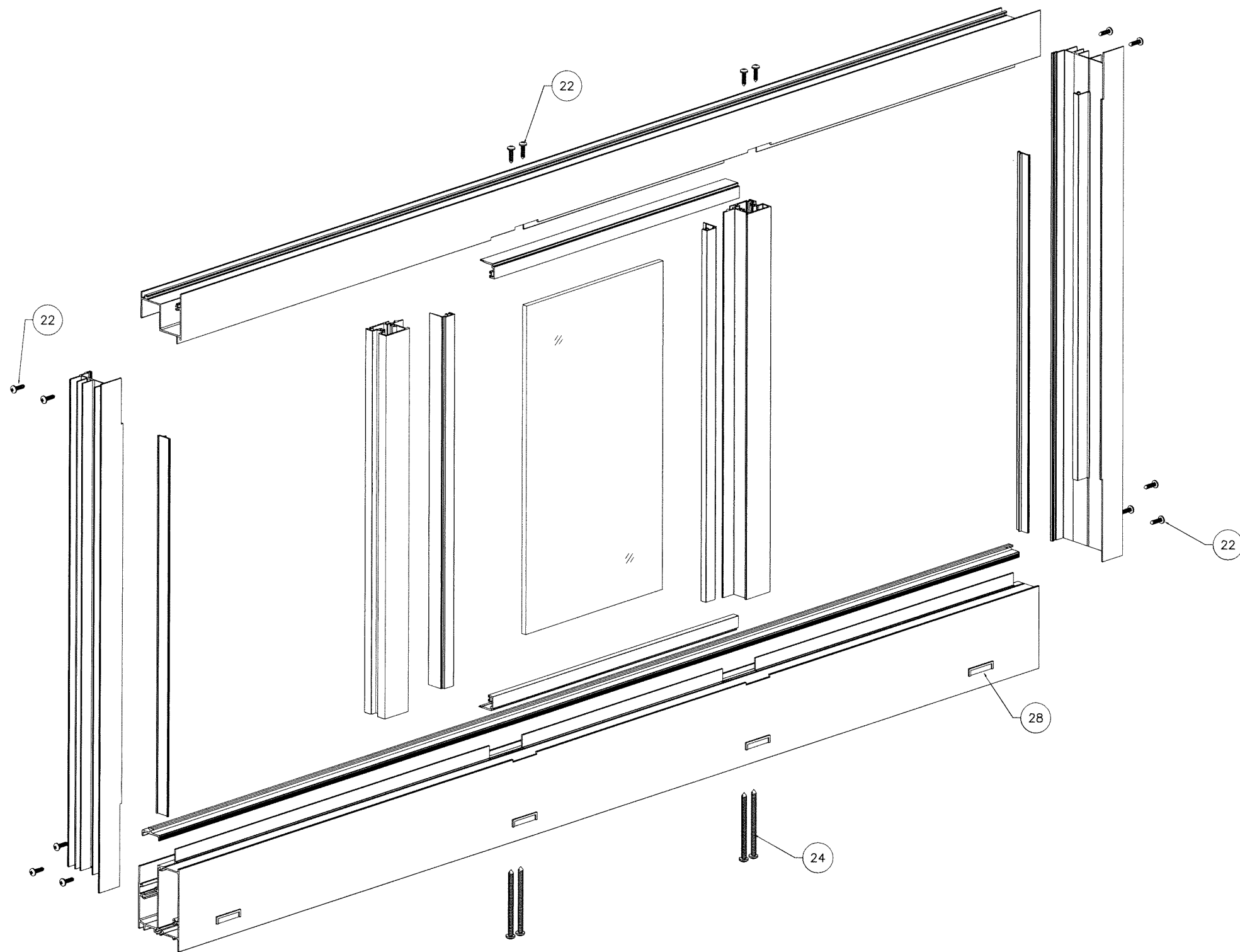
FRAME ASSEMBLY DETAIL
